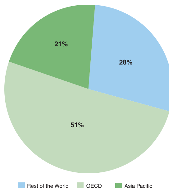
Figure 1.13: Share of World Energy Demand, 1992
