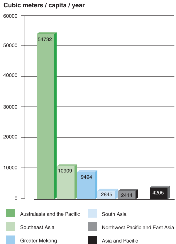
Figure 1.9: Renewable freshwater resources
