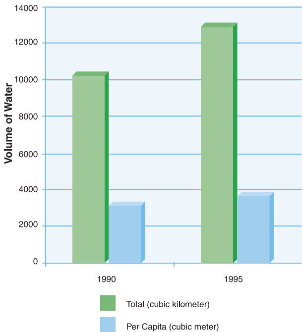
Figure 1.8: Annual Internal Renewable Water Resources in Asia, 1990 and 1995
