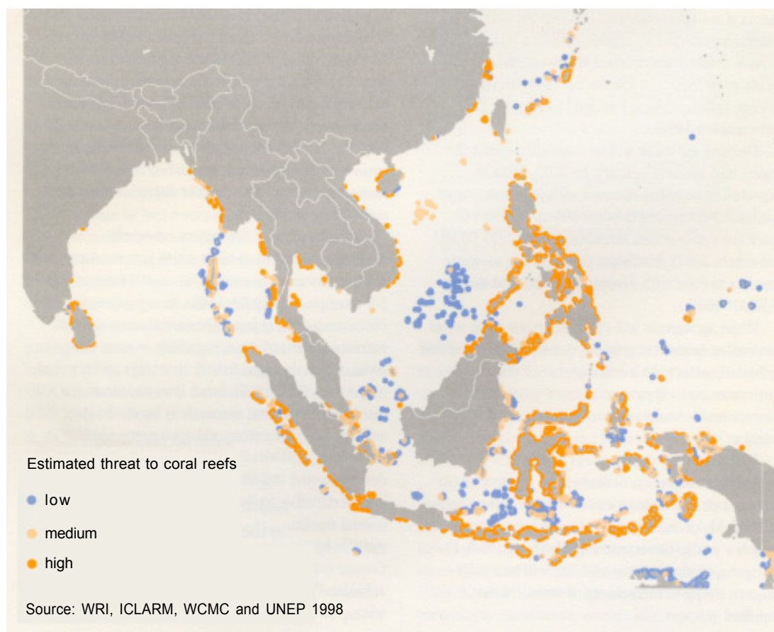
Figure 1.11: The threat to coral reefs
