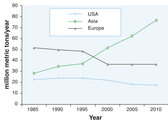
Figure 4.2: Current and Projected SO 2 Emissions
