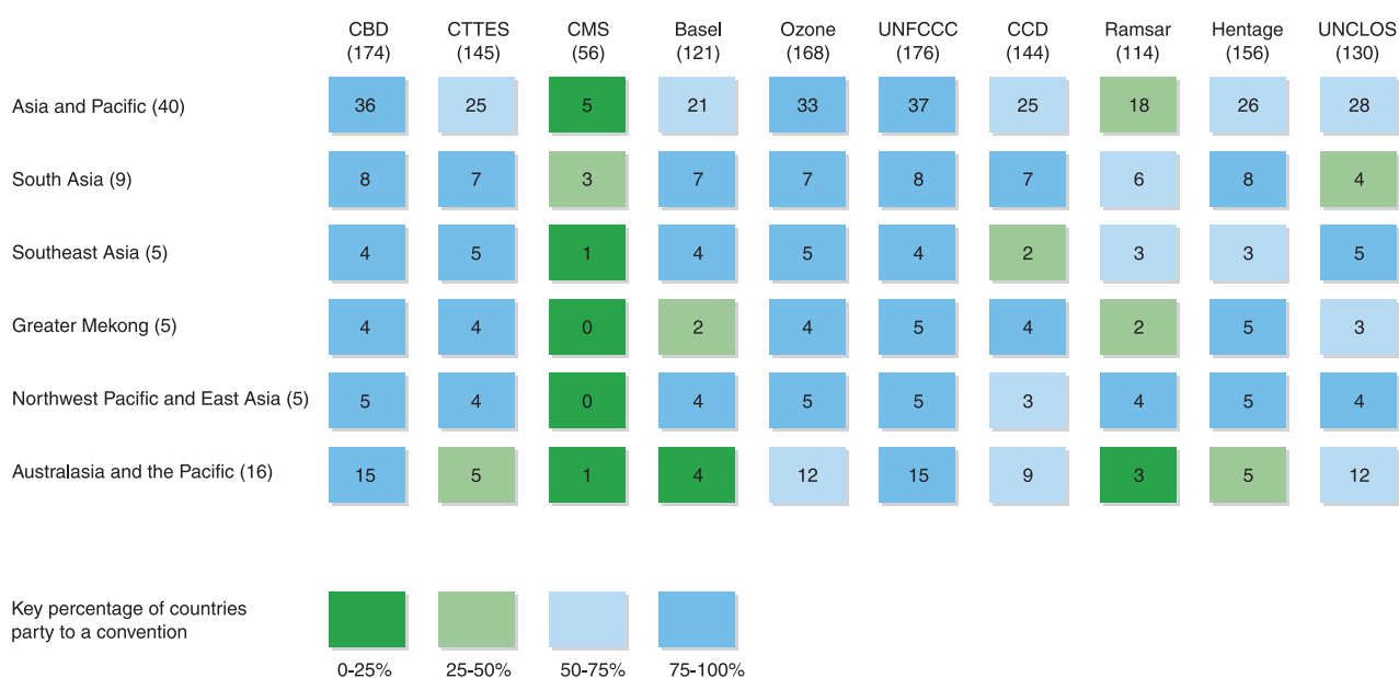
Figure 3.1: Parties to major environment conventions (as at 1 March 1999)
