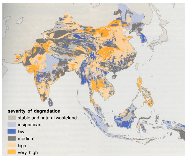
Figure 1.4: Severity of soil degradation in South and Southeast Asia
