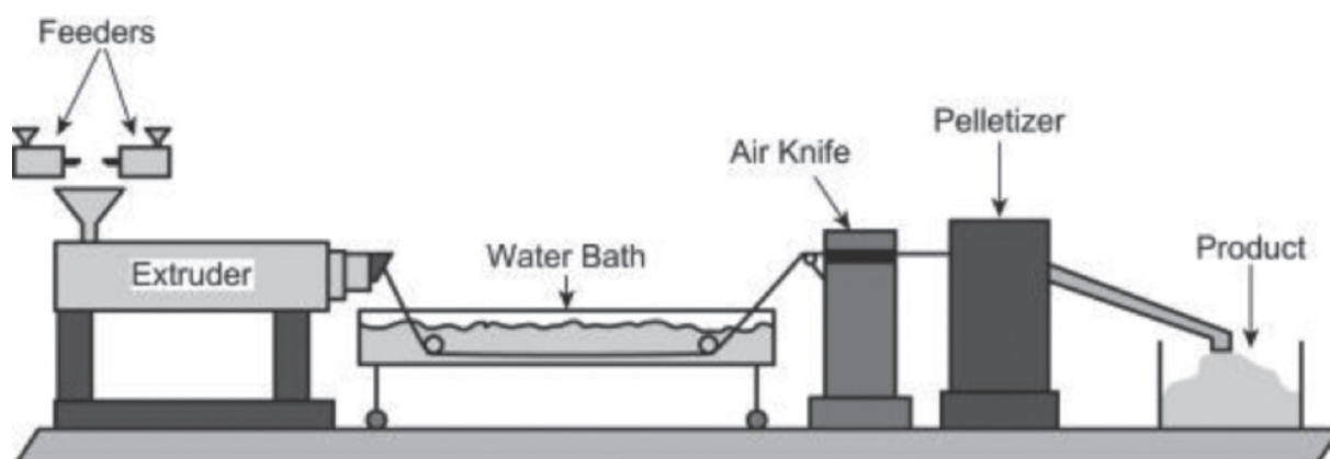
Figure 8. Compounding, extrusion and pelletizing process line 7
