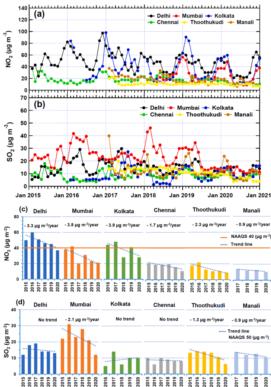
Fig. 4. Temporal variations in the concentration levels of NO_2 and SO_2 in Delhi, Mumbai, Chennai, Kolkata, Thoothukudi, and Manali from 2015 to 2020: (a) monthly NO_2 , (b) monthly SO_2 , (c) yearly NO_2 , and (d) yearly SO_2 . Trend analysis for yearly NO_2 and SO_2 and the government-prescribed National Ambient Air Quality Standards (NAAQS) for NO_2 and SO_2 are also included in the figure.
