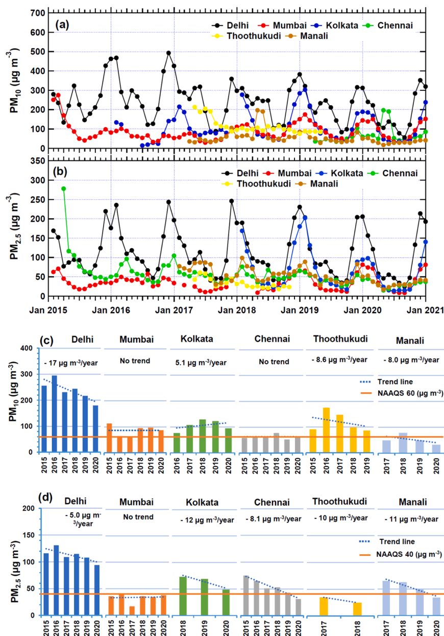
Fig. 3. Temporal variations in PM 10 and PM 2.5 concentration levels in Delhi, Mumbai, Chennai, Kolkata, Thoothukudi, and Manali from 2015 to 2020: (a) Monthly PM 10 , (b) Monthly PM 2.5 , (c) Yearly PM 10 , and (d) Yearly PM 2.5 . The figure also includes trend analysis for yearly PM 10 and PM 2.5 , along with the Government-prescribed National Ambient Air Quality Standards (NAAQS) for PM 10 and PM 2.5 .
