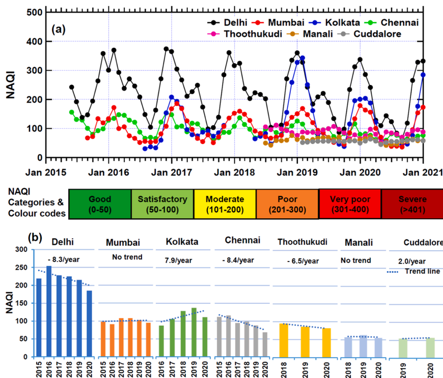
Fig. 5. Temporal variations in the concentration levels of NAQI in Delhi Mumbai, Chennai, Kolkata, Thoothukudi, Manali, and Cuddalore between 2015 and 2020: (a) monthly averaged NAQI (b) yearly averaged NAQI. Trend analysis for yearly NAQI is also included in the figure.
