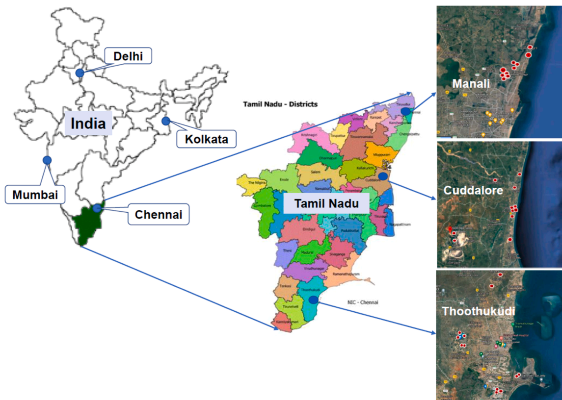
Fig. 1. Geographical location of Thoothukudi, Cuddalore, and Manali in Tamil Nadu. Additionally, the location of Delhi, Mumbai, Chennai, and Kolkata is also depicted in the figure. The red circles on the map indicate the presence of large industries in the industrial areas of Thoothukudi, Cuddalore, and Manali. Names of these industries and other major industries operated in Thoothukudi, Cuddalore, and Manali are given in Table 1.
